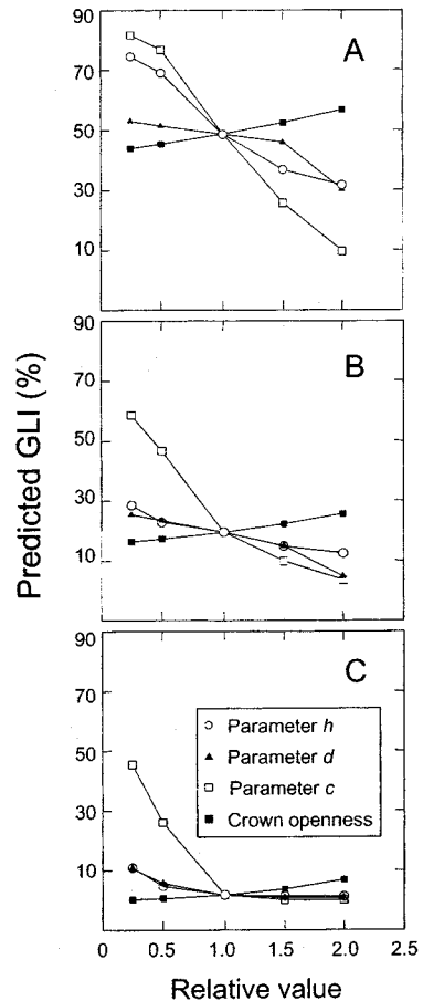
Fig. 1. Sensitivity of GLI predicted by SORTIE to variation in four parameters: h (which defines the relation between tree height and DBH), d (defining crown depth as a function of tree height), c (defining crown radius as a function of DBH), and crown openness. The sensitivity of the GLI predictions was assessed at a height of 1 m at three different locations in a stand: (A) north of a 400 \text{ m}^2 gap; (B) south of a 400 \text{ m}^2 gap; (C) under a closed canopy.
